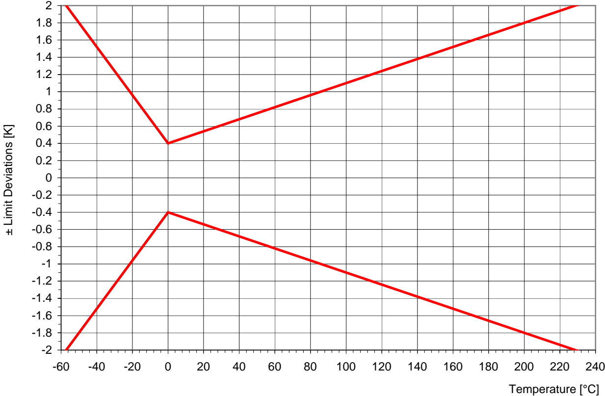
LG-Ni1000 Accuracy Tolerance according to DIN 43760, Class B
